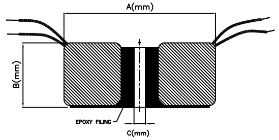
Dimensional drawing
